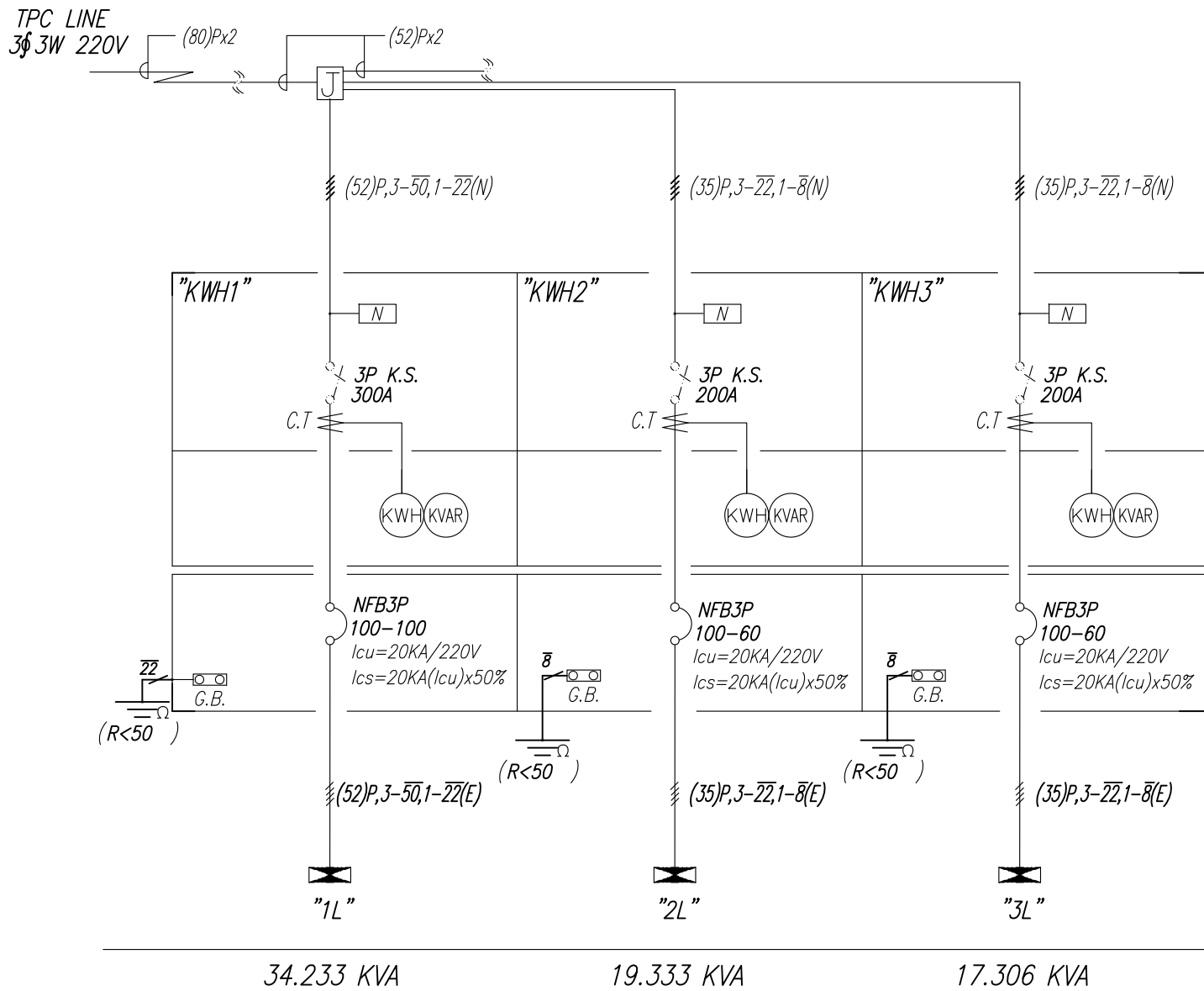
"KWH" 結線圖
