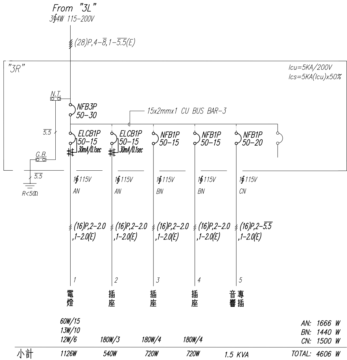
"3R" 結線圖 TOTAL: 4606 W I: 1666 W / 120V = 38.38 Amp
