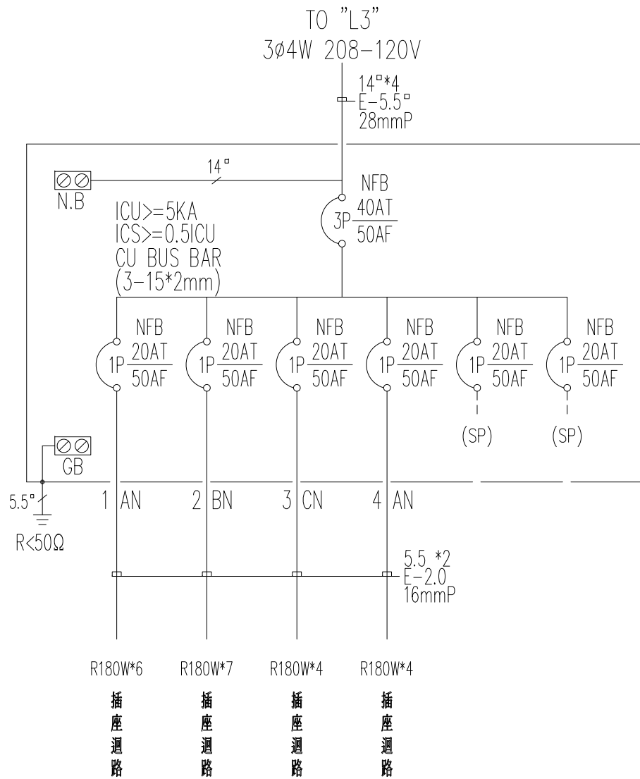
L4 PANEL LOAD: L=3.78KVA
