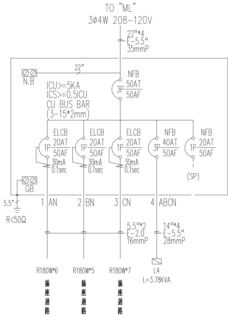
L3 PANEL LOAD: L=7.02KVA
