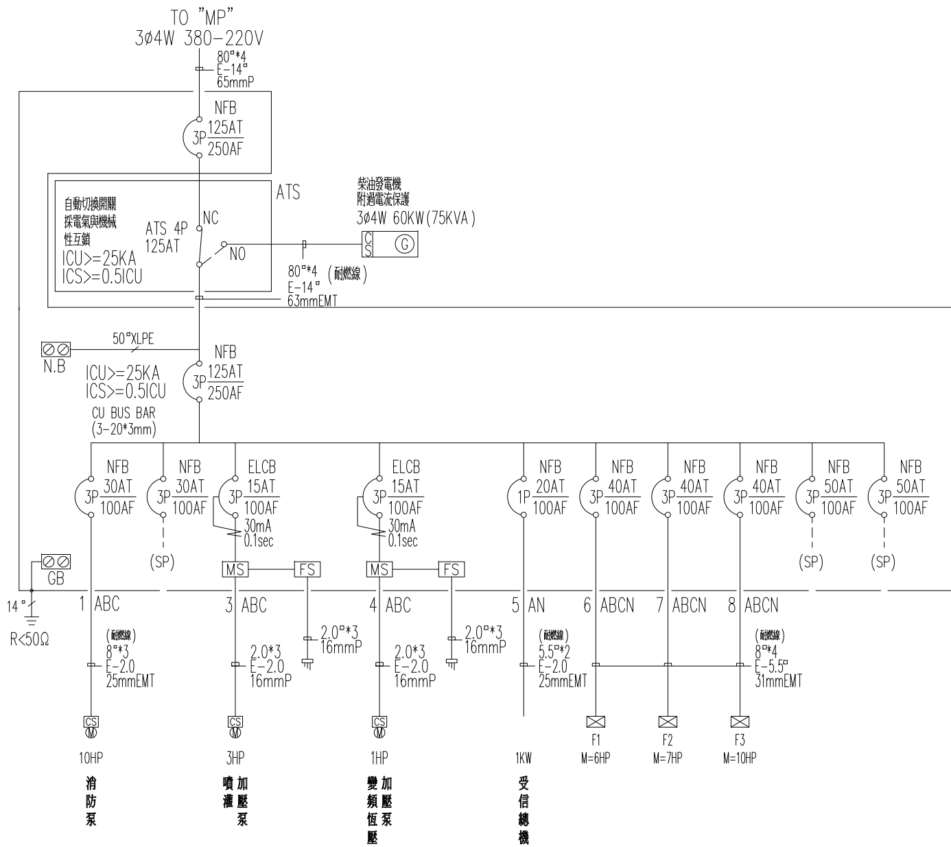
FP PANEL LOAD: M=37HP
