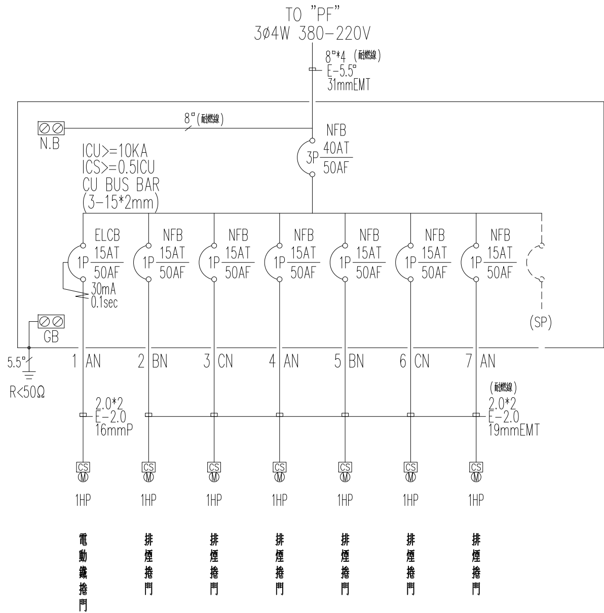
F2 PANEL LOAD: M=7HP
