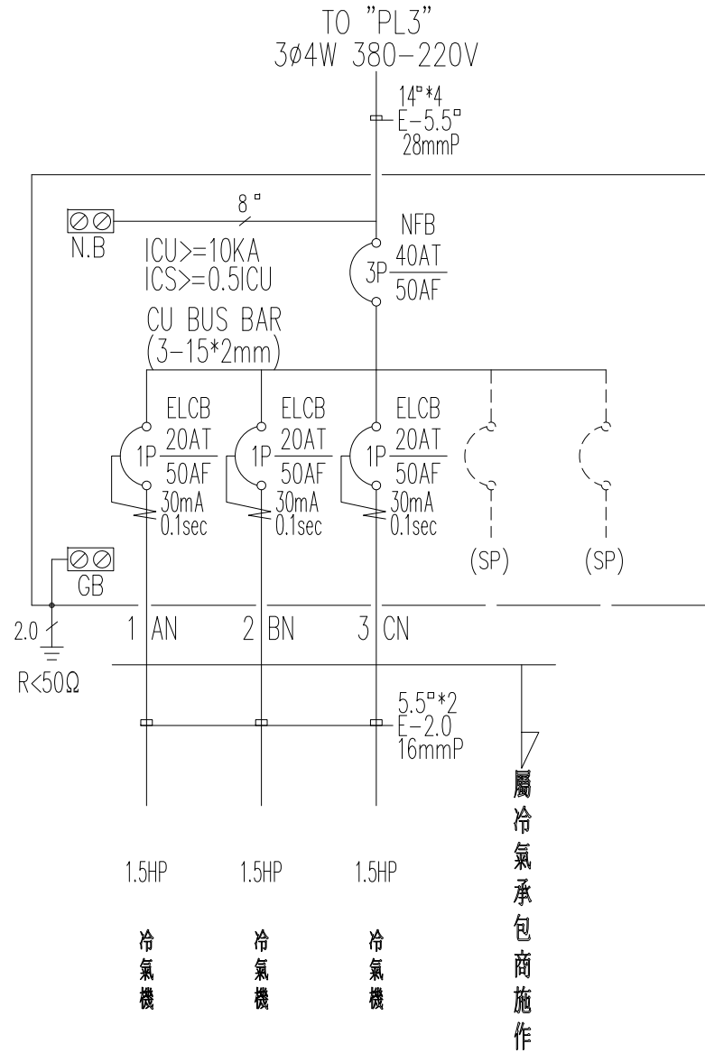
AC1 PANEL LOAD: M=4.5HP
